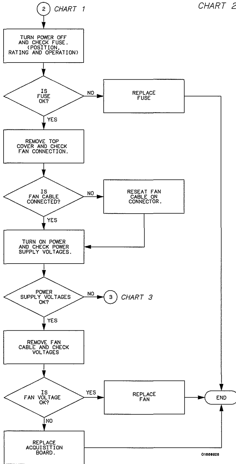
Troubleshooting Flowchart 2
