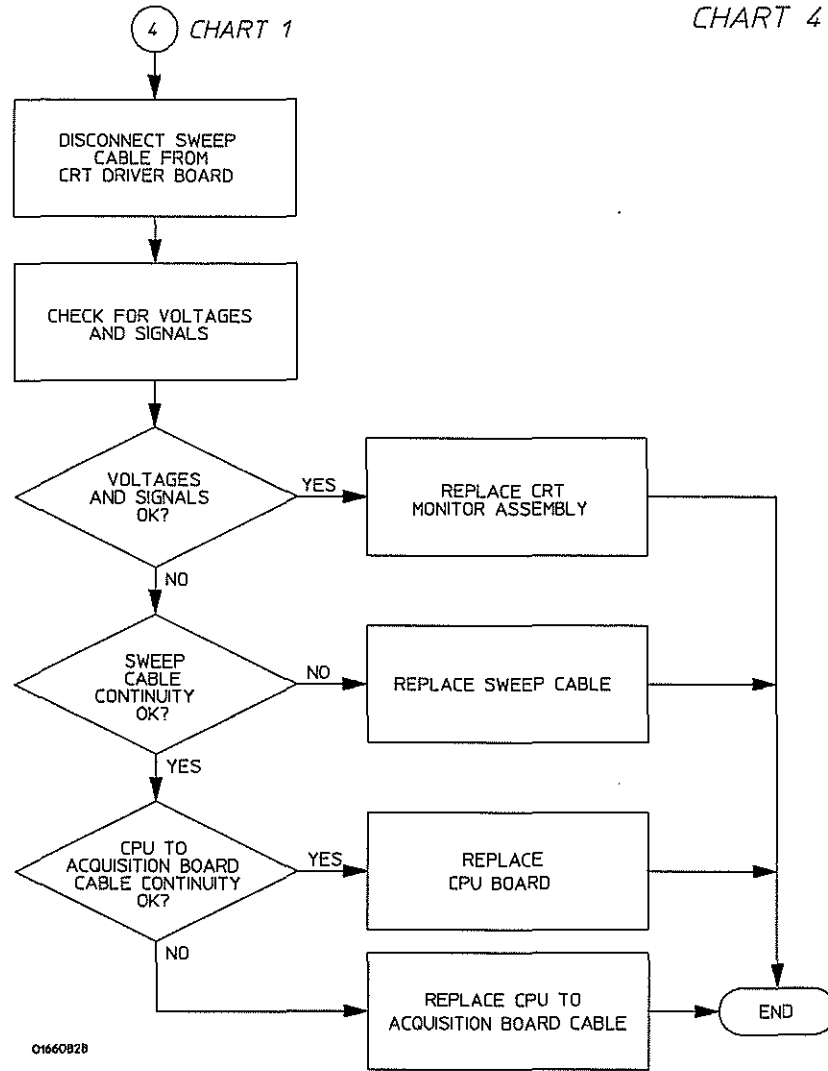
Troubleshooting Flowchart 4
