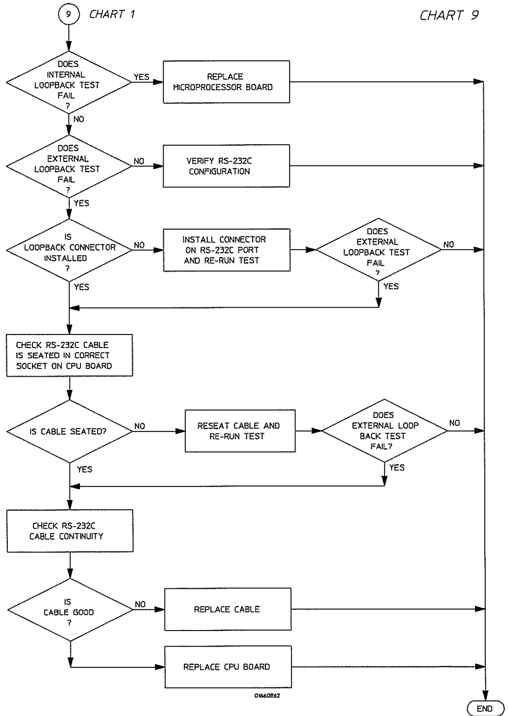
Troubleshooting Flowchart 9
