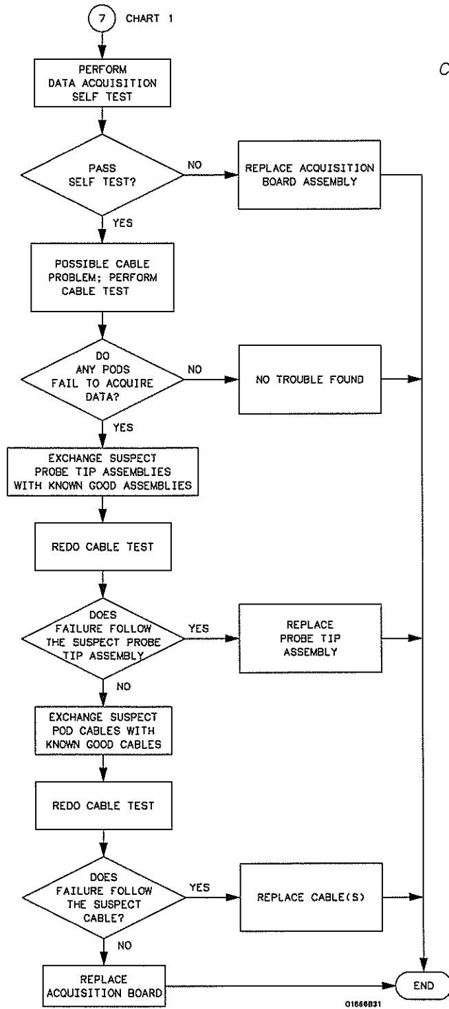
Troubleshooting Flowchart 7
