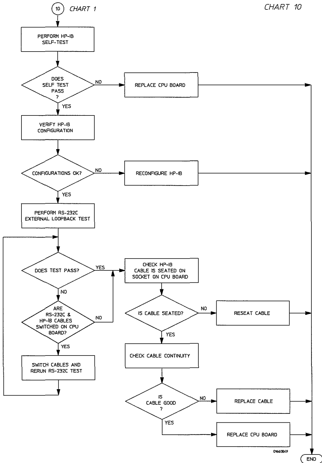
Troubleshooting Flowchart 10
