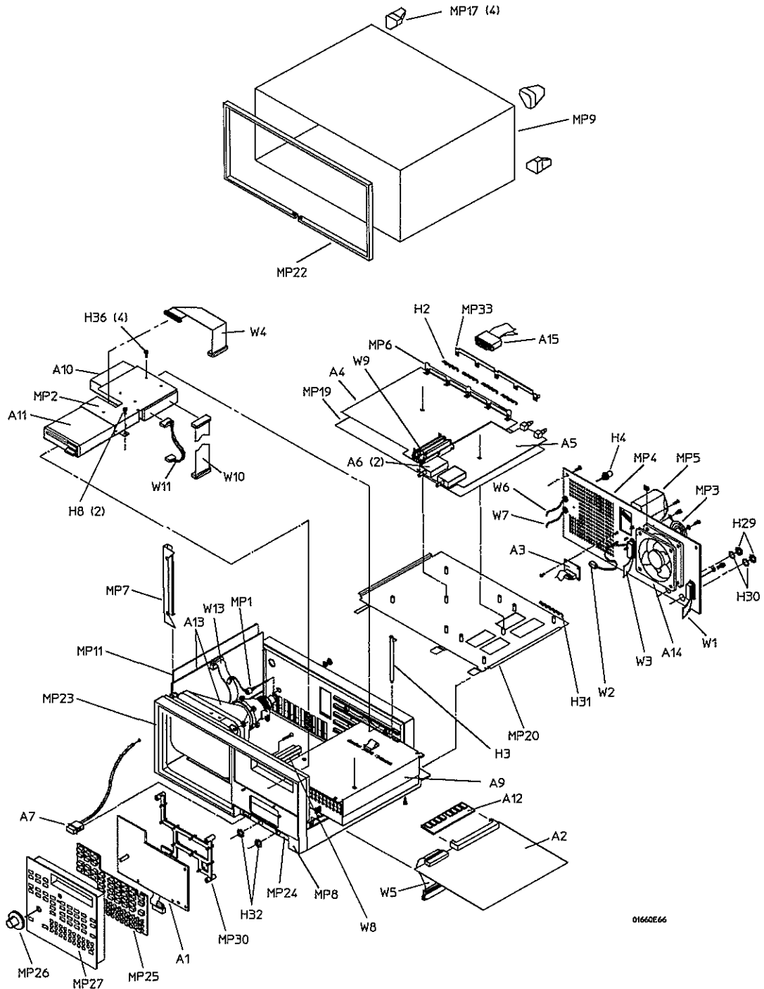
Exploded View of the HP 1660C
