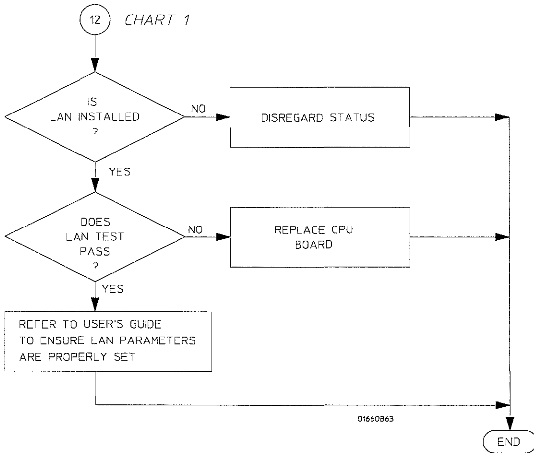
Troubleshooting Flowchart 12
