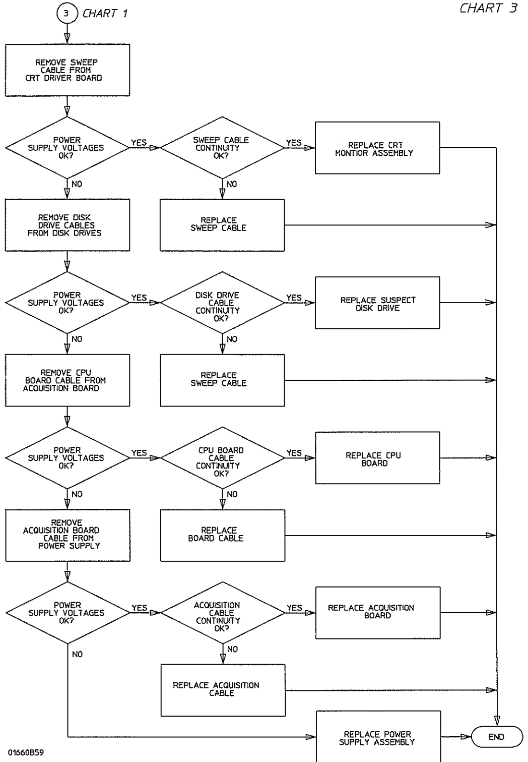
Troubleshooting Flowchart 3
