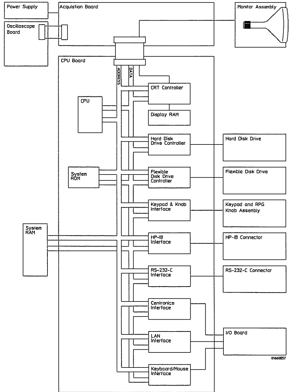
The HP 1660C/CS Logic Analyzer
